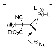
Figure 1. Mechanistic challenge of 2-quaternary palladium– \pi -allyl substitution.
